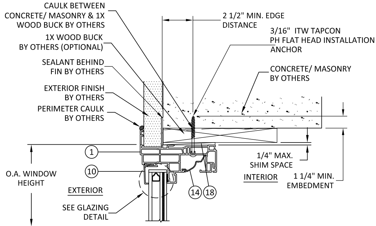
E 4 VERTICAL SECTION HEAD - CONCRETE/MASONRY J-CHANNEL/THROUGH FRAME
