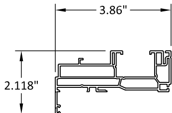
5 SILL RISER VINYL TYPICAL WALL THICKNESS: .060"
