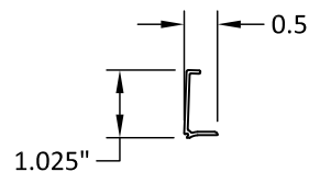
18 INSTALLATION CLIP STEEL
