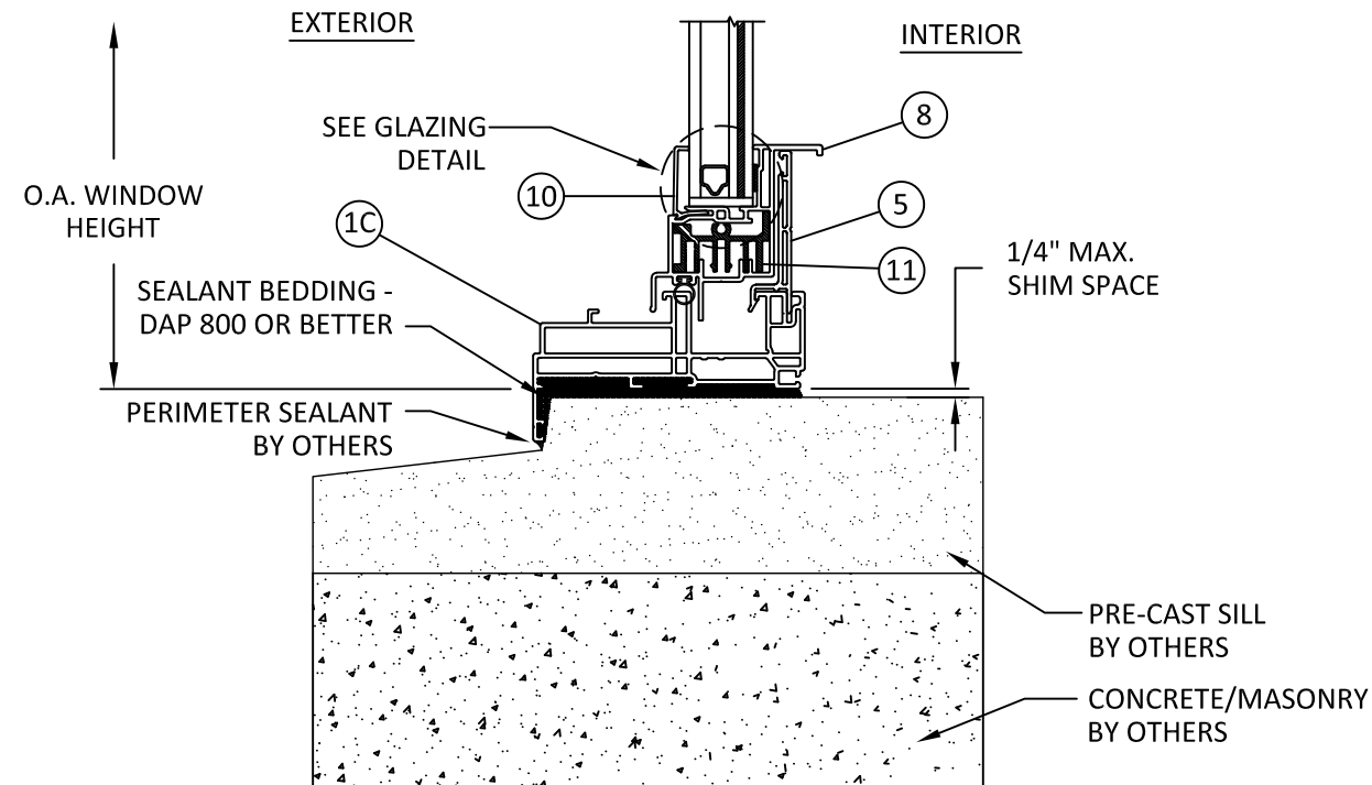
F 4 VERTICAL SECTION SILL - PRE-CAST SILL FLANGE/NO ANCHOR
