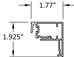
9 STILE VINYL TYPICAL WALL THICKNESS: .060"
