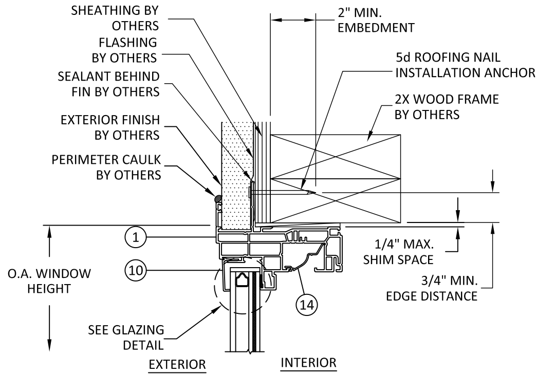
I 5 VERTICAL SECTION HEAD - 2X WOOD FRAME J-CHANNEL/NAIL FIN
