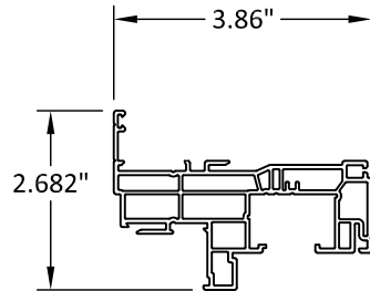
1B HEAD, JAMB FRAME (FLANGE) VINYL TYPICAL WALL THICKNESS: .060"
