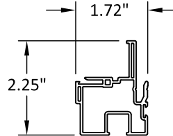
3 FIXED MEETING RAIL VINYL TYPICAL WALL THICKNESS: .050"
