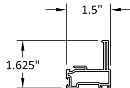
9 STILE VINYL TYPICAL WALL THICKNESS: .060"
