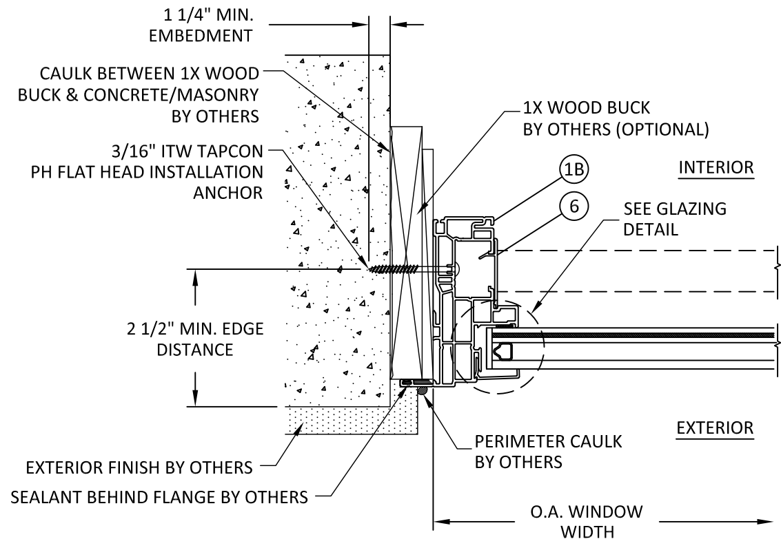
H 4 HORIZONTAL SECTION JAMB - CONCRETE/MASONRY FLANGE/THROUGH FRAME
