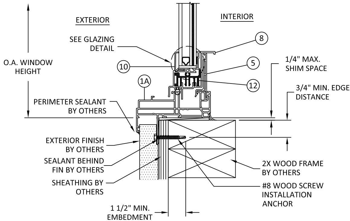
J 5 VERTICAL SECTION SILL - 2X WOOD FRAME J-CHANNEL/NAIL FIN
