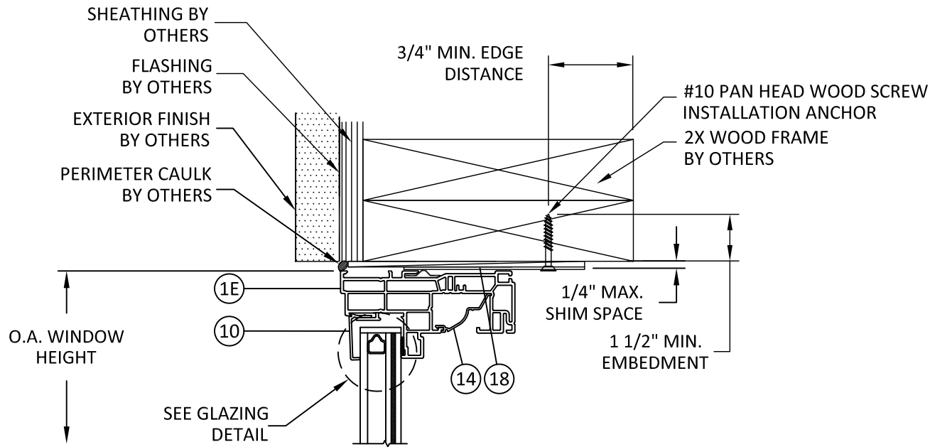
A 3 VERTICAL SECTION HEAD - 2X WOOD BUCK REPLACEMENT/INSTALLATION CLIP
