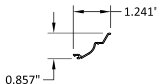
14 BALANCE COVER VINYL TYPICAL WALL THICKNESS: .040"
