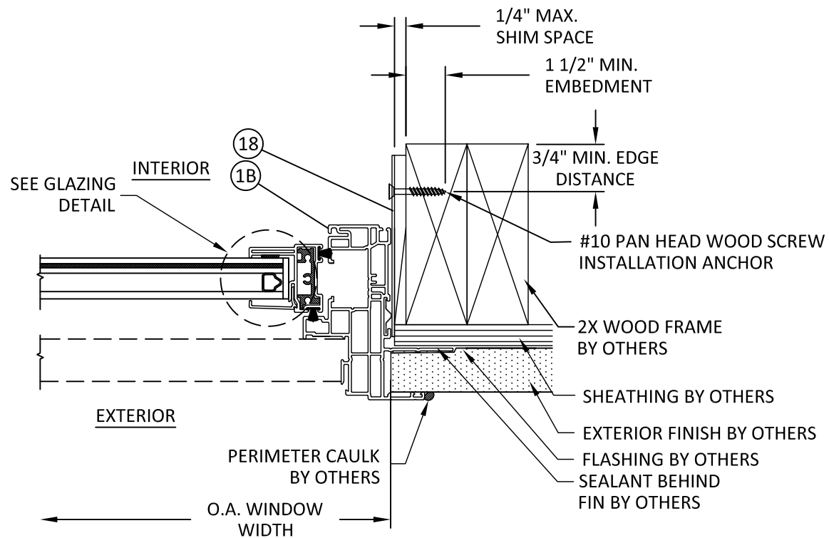
C 3 HORIZONTAL SECTION JAMB - 2X WOOD FRAME J-CHANNEL/INSTALLATION CLIP
