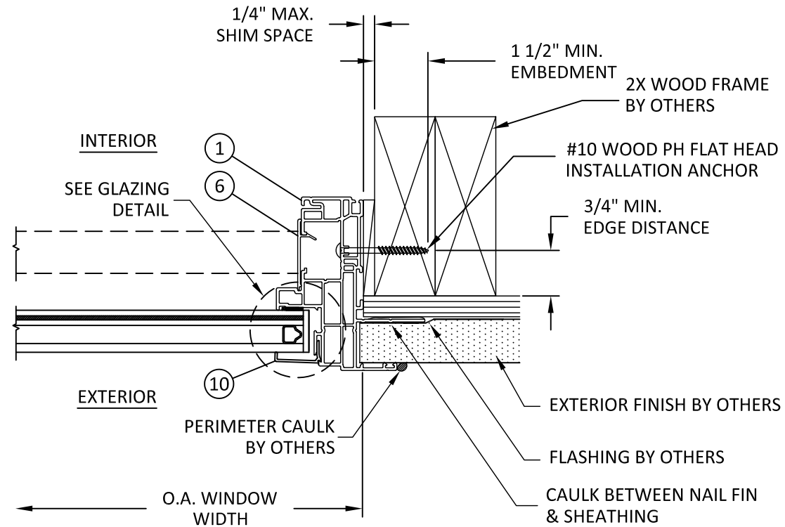
G 4 VERTICAL SECTION JAMB - WOOD J-CHANNEL/THROUGH FRAME
