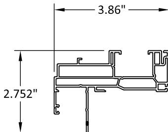
1A SILL FRAME (FIN) VINYL TYPICAL WALL THICKNESS: .060"
