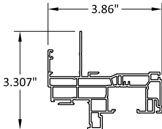
1 HEAD, JAMB FRAME (FIN) VINYL TYPICAL WALL THICKNESS: .060"
