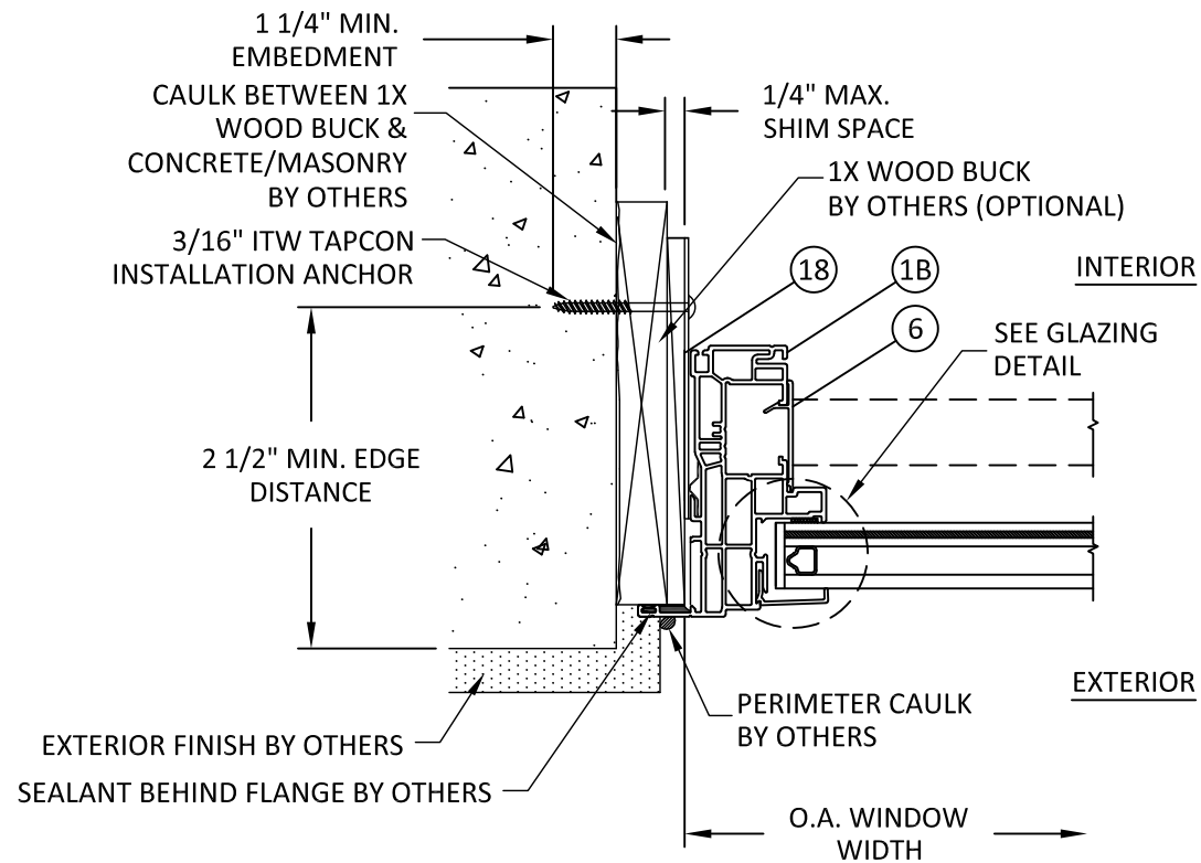
D 3 HORIZONTAL SECTION JAMB - CONCRETE/MASONRY FLANGE/INSTALLATION CLIP
