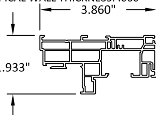
8 LIFT RAIL VINYL TYPICAL WALL THICKNESS: .060"
